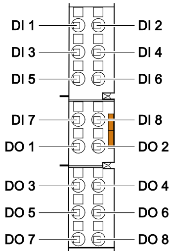
Figure 4: CAGE CLAMP® S Connectors
