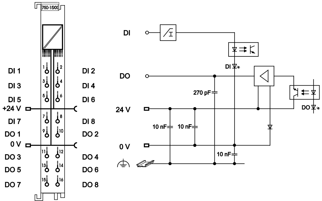
Figure 6: Schematic Diagram
